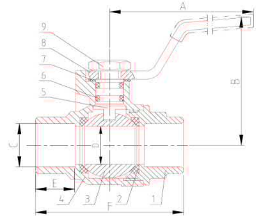
702 Solder Series
