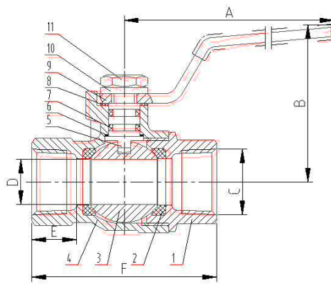
701 Threaded Series
